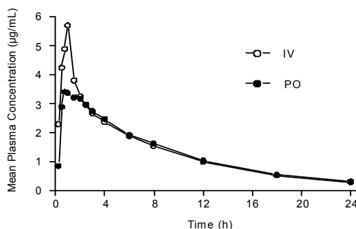
Figure 1: Mean Plasma Concentration-Time Profiles of Gatifloxacin Following Intravenous (IV) and Oral (PO) Administration of a Single 400-mg Dose to Healthy Subjects.
